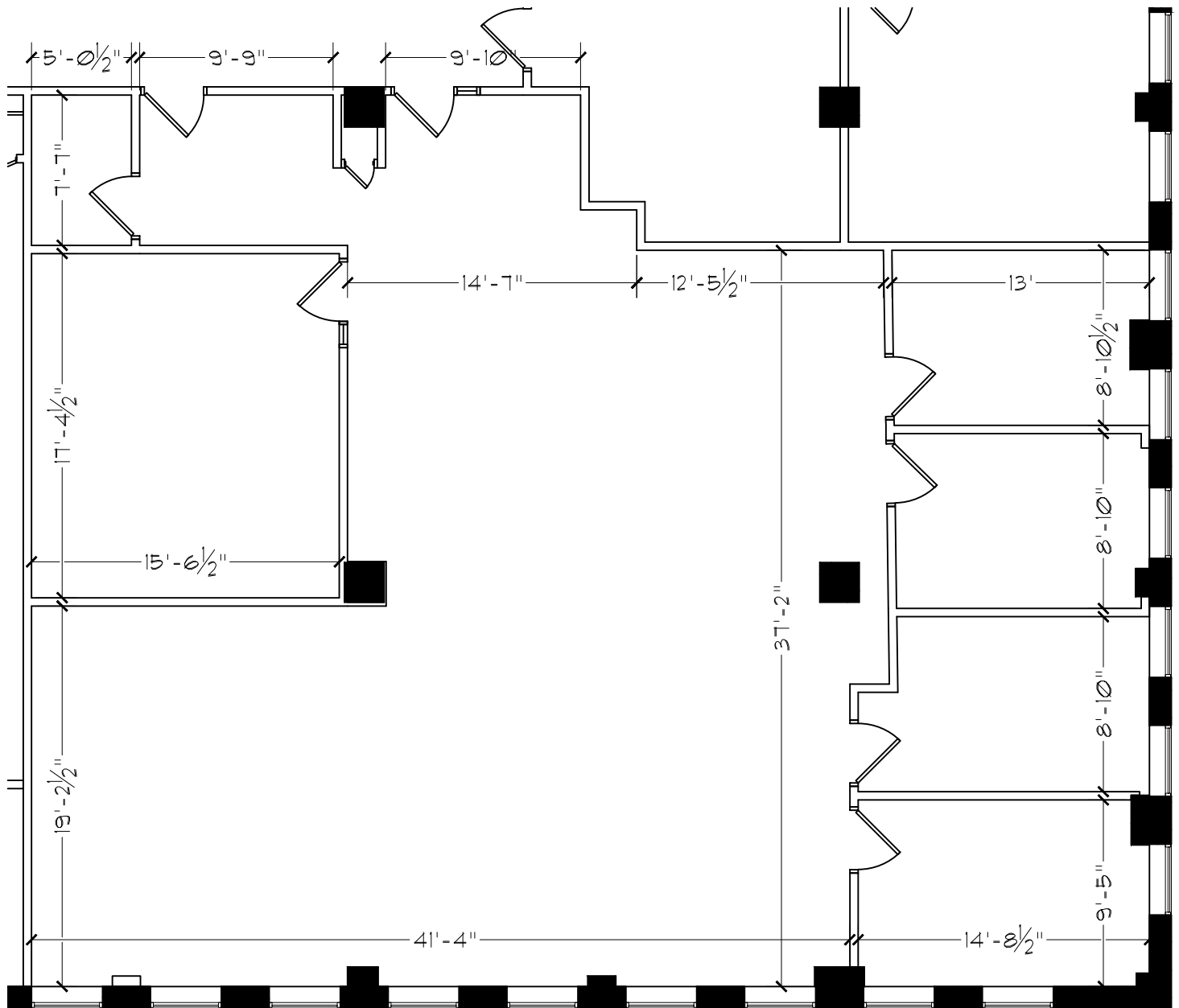
KEY PLAN - 3rd FLOOR
