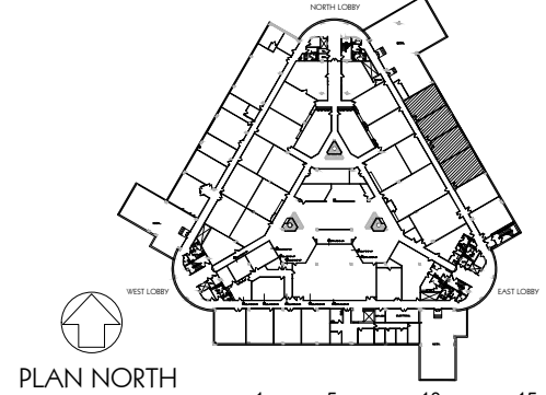
KEY PLAN - LOWER LEVEL
