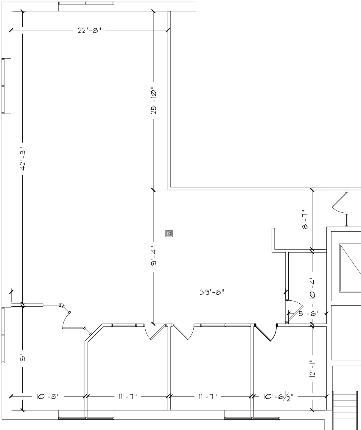
KEY PLAN - 1ST FLOOR
